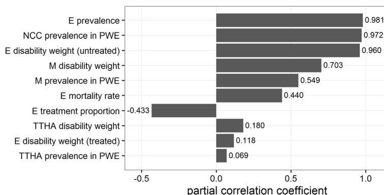
Fig. 3 Partial correlation coefficients showing which parameter influences the estimated DALYs due to NCC-associated epilepsy, migraine and tension-type headache for the year 2007 in Angónia district, Mozambique. E-epilepsy; NCC-neurocysticercosis; PWE-people with epilepsy; M-migraine; TTHA-tension-type headache
